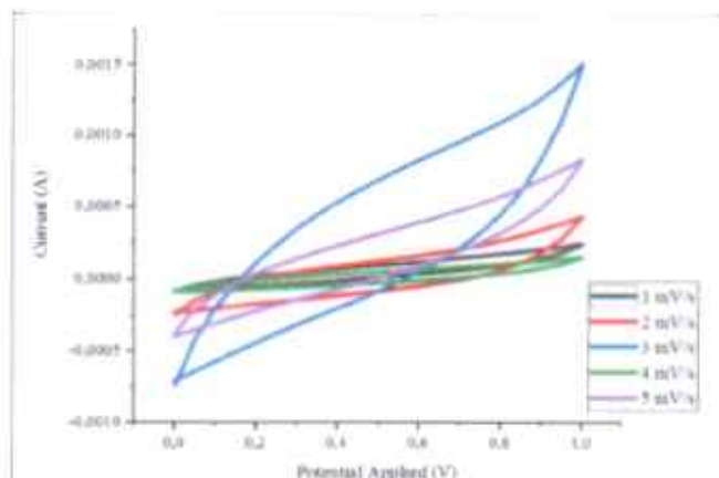
Figure 3. Cyclic voltametric curve of Activated Carbon/rGO composite electrode (90/10 wt%) with scan rate variation 1-5 \text{mVs}^{-1} , potential range 0 - 1 V in 1M \text{Na}_2\text{SO}_4 electrolyte solution.
